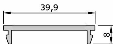
*10204 0,275 kg/m Plug for Sash
