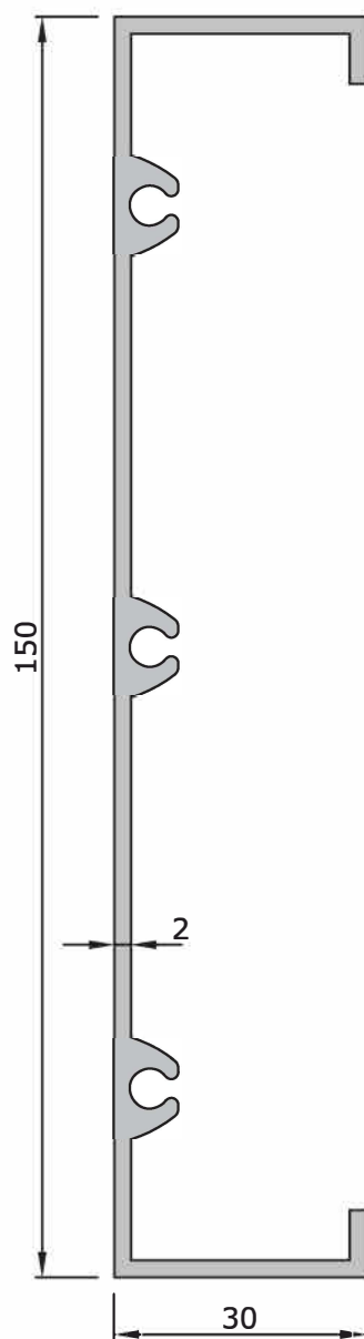
3281* 1,450 kg/m | 150 mm Frame Profile
