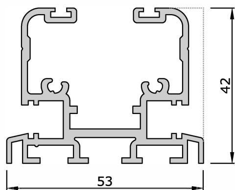
5963 1,225 kg/m Guide For Sash (Bottom)
