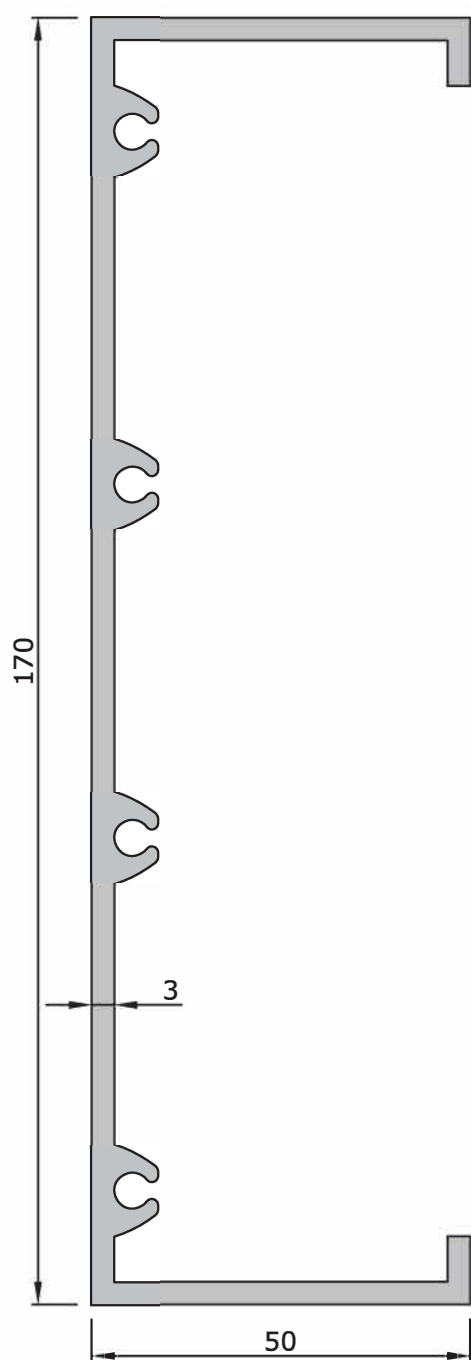
3294* 2,620 kg/m | 170 mm Frame Profile
