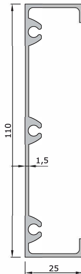
3481* 0,965 kg/m | 110 mm Frame Profile
