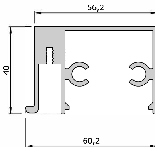
*10203 1,565 kg/m Sash Profile (Transom-for Upper and Bottom)
