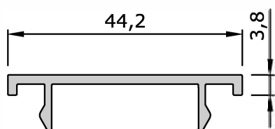
8962 0,300 kg/m Plug for Sash
