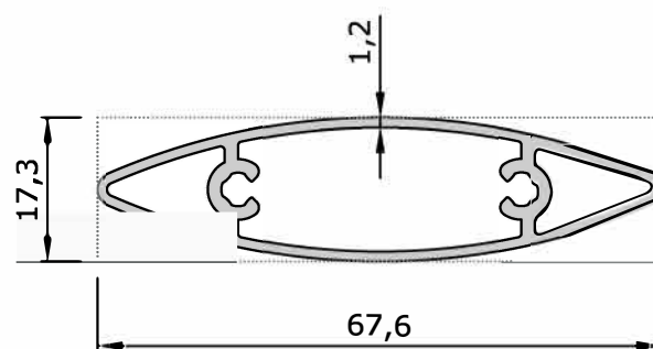
8960 0,620 kg/m 67,6 mm Sunbreaking Profile
