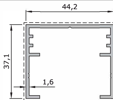
10409 0,610 kg/m | Frame Profile
