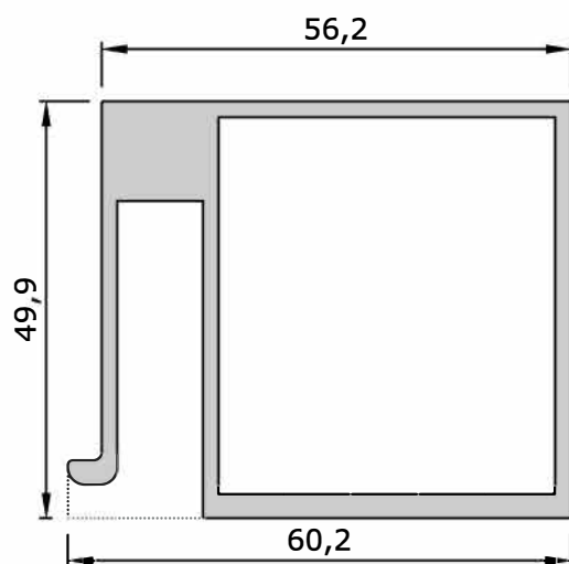
*10202 1,625 kg/m Sash Profile (Mullion)
