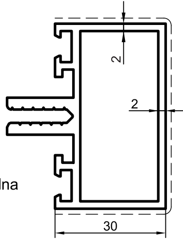
30' Horizontala 1,210 kg/m J_x = 10,54 \text{ cm}^4 J_y = 7,20 \text{ cm}^4
